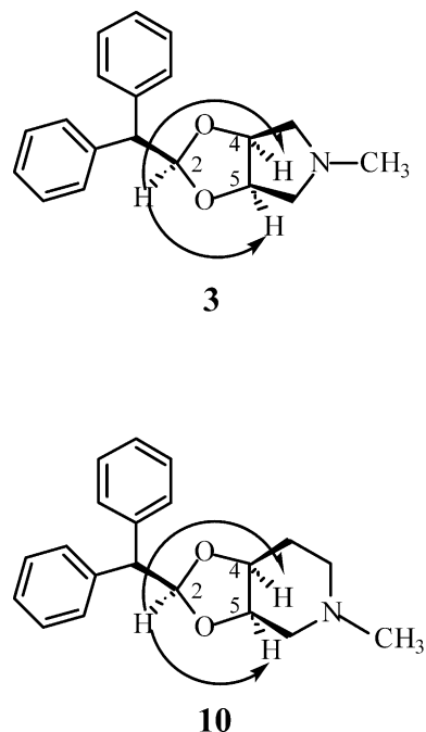
Figure 1. Principal correlations observed in the NOE spectrum of compounds 3 and 10 . The numeration refers to the dioxolane cycle and not to the bicyclic one.
