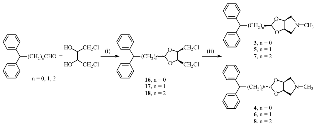
Scheme 1. (i) TsOH, (ii) CH 3 NH 2 .
