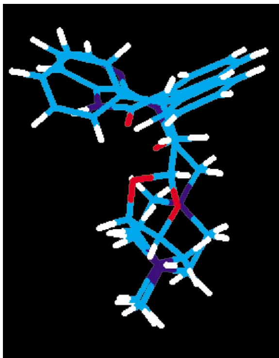
Figure 2. Overlay of pirenzepine and compound 6 .
